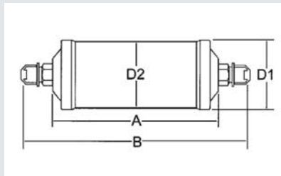
Flare Connection
